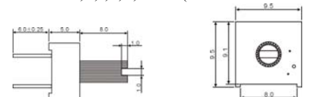
TSR-3386F,K,P,R,U,Y-EY5 (RESISTANCE CODE)-TL
