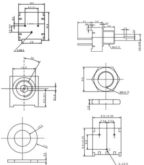
TSR-3386F,K,P,R,U,Y-EY5 (RESISTANCE CODE)-TL
