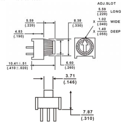
TSR-3386F,K,P,R,U,Y-EY5 (RESISTANCE CODE)-L
